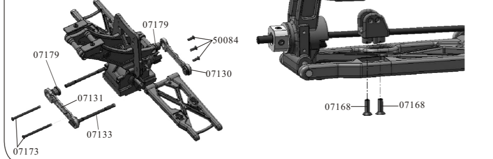
Rear lower Suspension Arms Assembly
