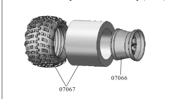
Wheels Complete Assembly
