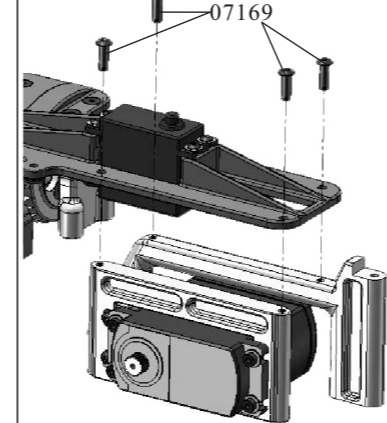
Throttle Link Assembly
