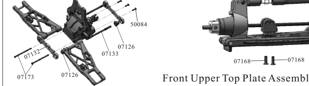
Front Upper Suspension Arms Assembly
