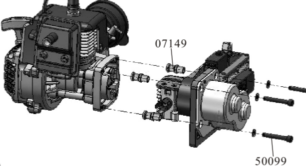
Center Unit Assembly
