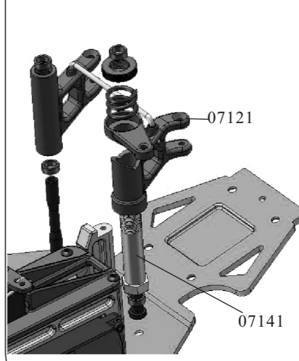
Buffer Assembly
