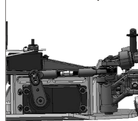
Servo link Assembly
