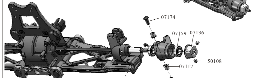
Steering Mount Assembly
